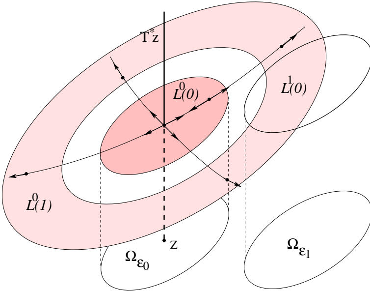
Figure 3.1. Sketch of the Lagrangian manifold \mathcal{L}_{\eta_1}^0(0) situated above \Omega_{\epsilon_0} and centered at z (center ellipse, dark grey), its image \mathcal{L}_{\eta_1}^0(1) through the flow (external annulus, light grey) and the intersection \mathcal{L}_{\eta_1}^1(0) of the latter with T^*\Omega_{\epsilon_1} . The thick arrows show the possible momenta at points x \in M (black dots).
