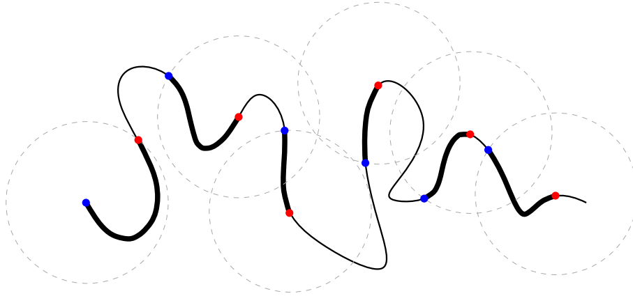
FIGURE 3.7. Illustration of the procedure (P_\alpha) . The times \sigma_i are in blue, and the \tau_i in red. Several subpaths (in thick line), spanning a distance \delta and being \alpha\delta apart, are created from the initial path. The balls have radius \delta .
