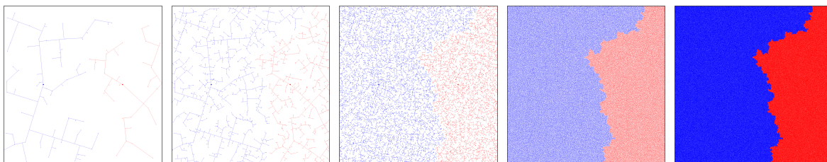
FIGURE 1.2. Simulation of the variant Poisson coloring of space where a new incoming point is linked by a monochromatic segment to the nearest point in the process so far, from left to right with 10^2, 10^3, 10^4, 10^6 and 10^7 points. The arrivals points X_i are the same as those used for Figure 1.1. Notice that the red “island” on the top right part of the figure present in the original point model has disappeared.
