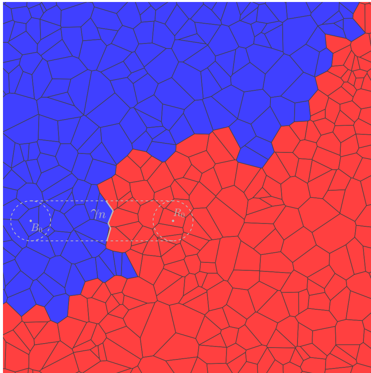
FIGURE 3.8. Colored Voronoi diagram of the points R_0, B_0, X_1, \dots, X_n . Balls with radius r/2 are represented around R_0 and B_0 . The path \gamma_n is also represented, and it has diameter at least r .
