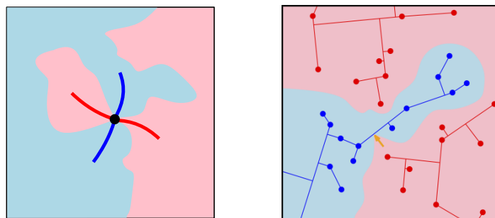
FIGURE 1.4. Left. Illustration of a double point in the frontier \mathcal{F}_\infty . Right. Can the frontier intersect the finite trees in the segment model (orange arrow)?
