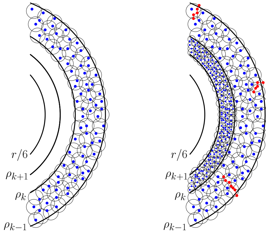
FIGURE 2.6. Schematic description of the induction procedure.
