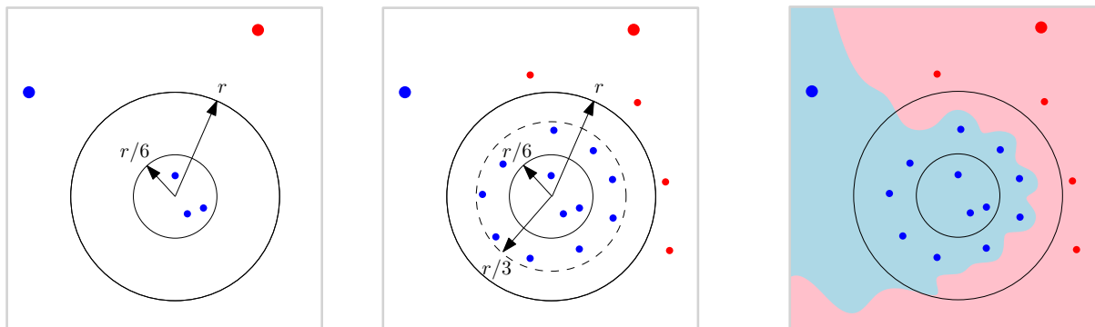
FIGURE 2.5. Illustration of the construction of the event G_{r/6,r}^x . Suppose that the seeds R_0, B_0 lie outside \bar{B}(x, r) .
