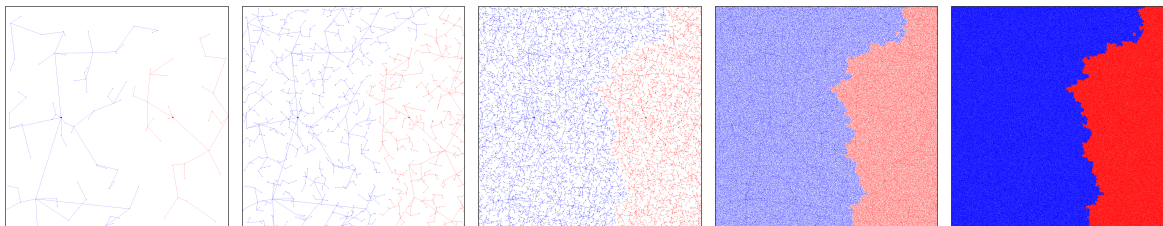
FIGURE 1.1. Simulation of the Poisson coloring of space where a new incoming point takes the color of the nearest neighbor in the process so far, from left to right with 10^2 , 10^3 , 10^4 , 10^6 and 10^7 points.
