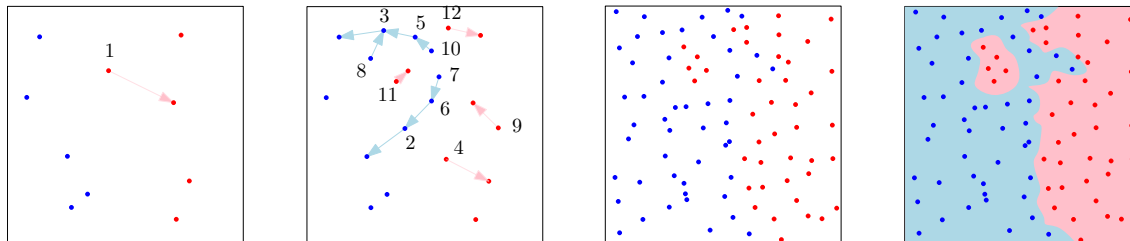
FIGURE 1.3. Illustration of the creation of an “island”. Such an island can be seen on Figure 1.1 on the top right corner. This shows that the limiting frontier \mathcal{F}_\infty is not connected almost surely.
