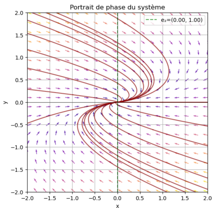
FIGURE 13.5 – D = \begin{pmatrix} -0.6 & 1 \\ 0 & -0.6 \end{pmatrix} ; P = I_2
