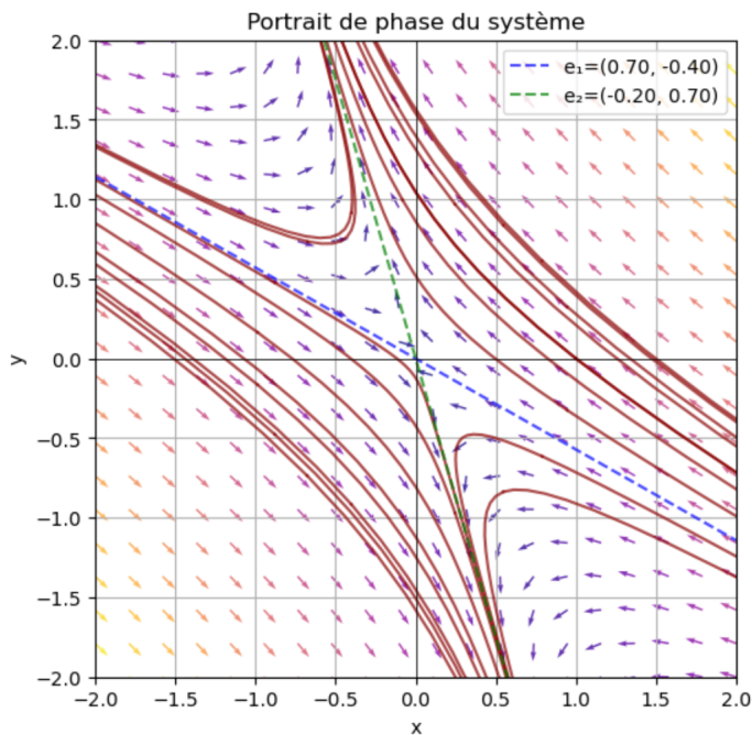
FIGURE 13.4 – D = \begin{pmatrix} 2 & 0 \\ 0 & 1 \end{pmatrix} ; P = \begin{pmatrix} 0.7 & -0.2 \\ -0.4 & 0.7 \end{pmatrix}
