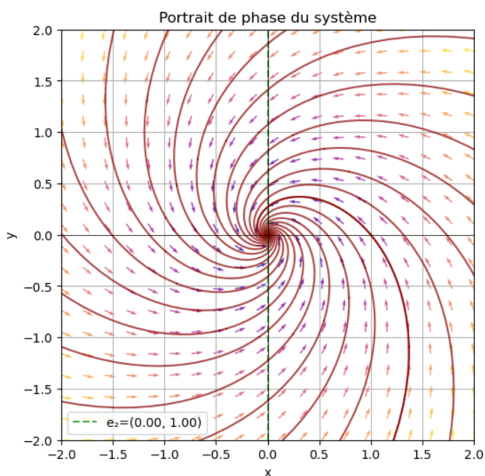
FIGURE 13.7 – D = \begin{pmatrix} -0.5 & -0.6 \\ 0.6 & -0.5 \end{pmatrix} ; P = I_2
