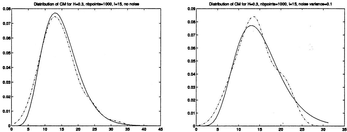
Figure 3.3 : Empirical statistics compared with the corresponding \chi^2_{l-2}
