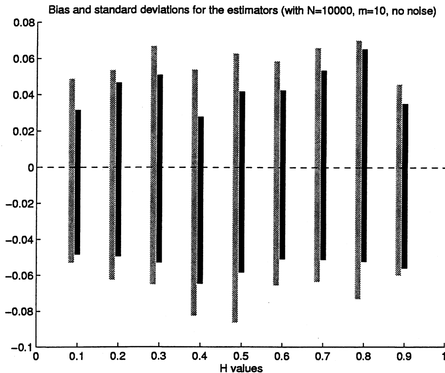
Figure 4.1 : Estimators of H for f.B.m. (from left to right \widehat{H}_1 and \widehat{H}_2 ) for each value of H
