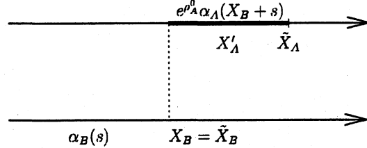
Figure 2.2: Case X_B < X_A : \tilde{X}_A = X_B + X'_A
