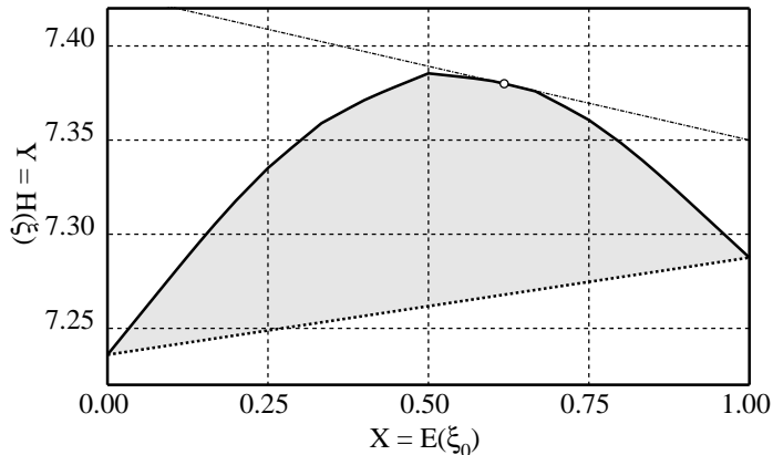
Figure 3: The set \mathcal{P} = p[\text{St}(I)] , for h_0 = 0.6 , h_1 = 0.7 and \kappa = 0.1
