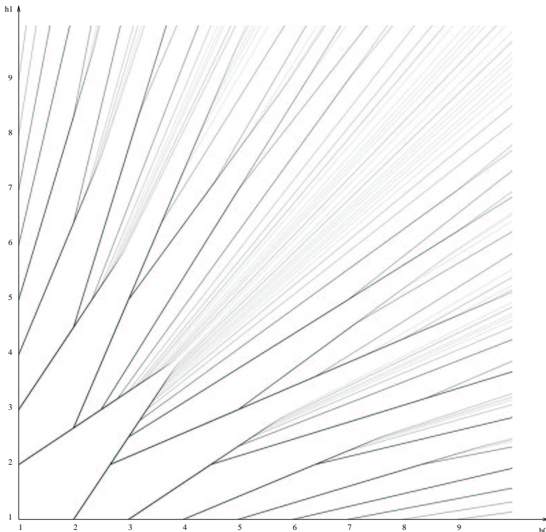
Figure 2: The Tetris phase diagram
