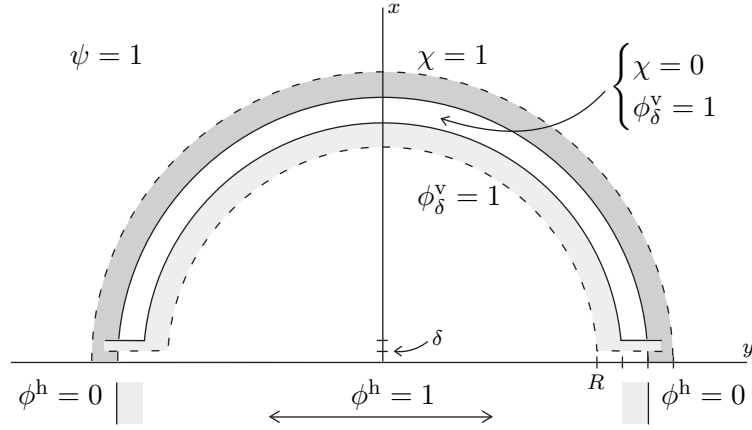
FIGURE 3. Structure of cutoffs in the model cusp neighbourhood (with the z coordinate suppressed). The supports of \nabla\phi^h and \nabla\phi_\delta^v are light gray and the support of \nabla\chi is dark gray. The entire picture is contained within the support of \psi .
