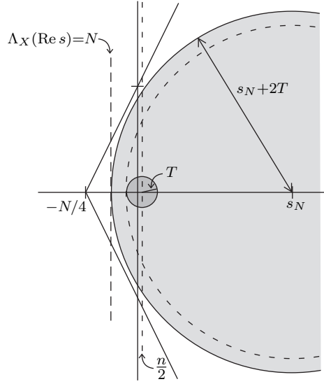
FIGURE 5. The big disk in which Jensen's inequality is applied, centered at s_N , containing the disk of radius T centered at n/2 in which the resonances are counted.
