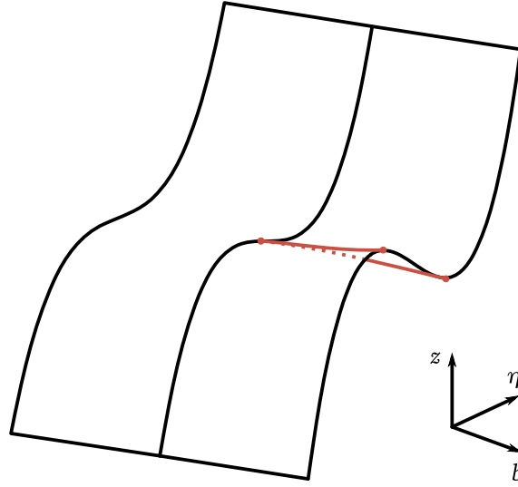
Figure 14. Graph of the generating family f_z^1 with fibrewise critical values in red.
