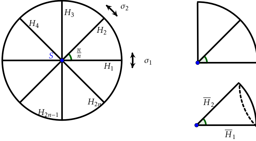
Figure 2: A n -dihedral manifold M , its fundamental piece and the quotient \overline{M} .
