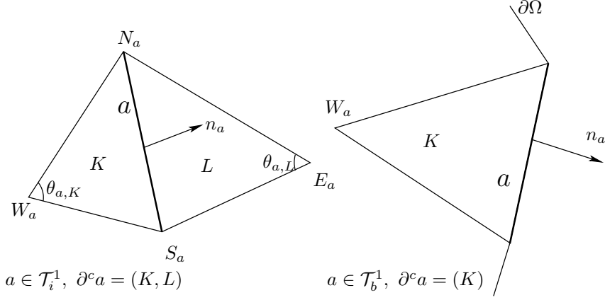
Figure 2: Mesh notations for an internal edge (left) and for a boundary edge (right)
