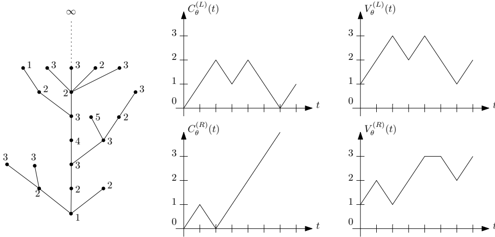
Figure 2: An infinite well-labeled tree \theta and its contour functions (C_\theta^{(L)}, V_\theta^{(L)}) , (C_\theta^{(R)}, V_\theta^{(R)}) .
