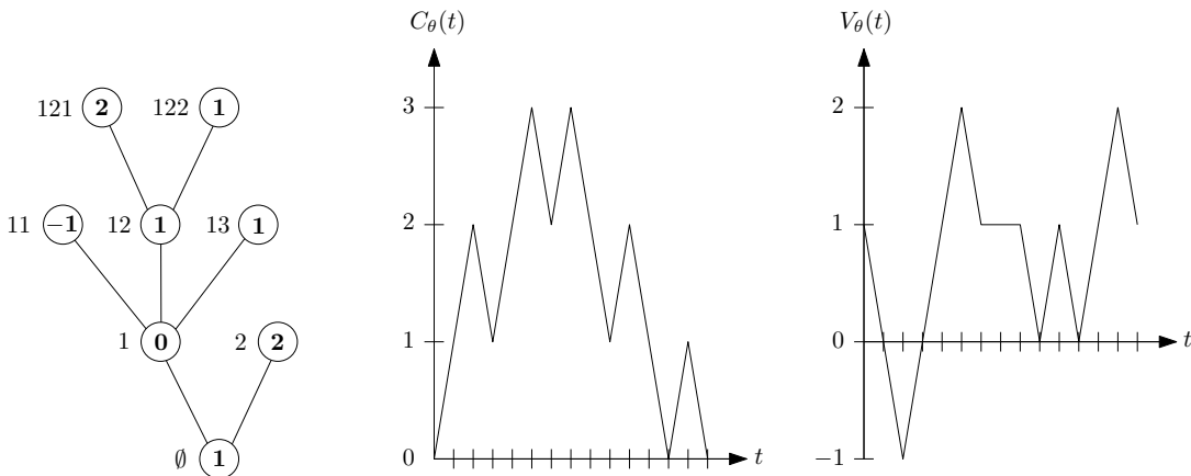
Figure 1: A labeled tree \theta and its pair of contour functions (C_\theta, V_\theta) .
