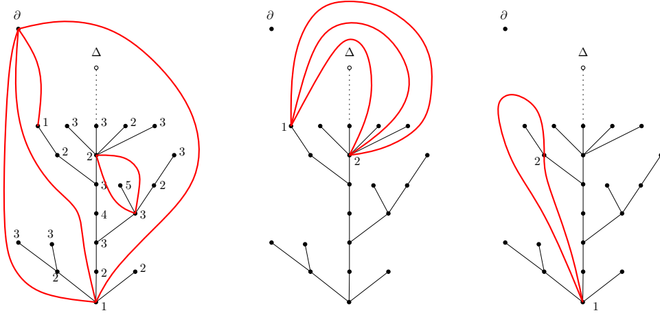
Figure 3: Construction of a few edges in Schaeffer's correspondence.
