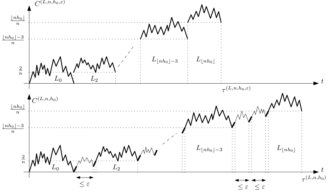
Figure 4: The processes C^{(L,n,h_0)} and C^{(L,n,h_0,\varepsilon)} .
