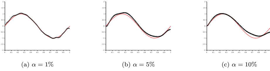
Fig. 10: Recovery of the potential Q(x) = \sin(\pi x) in presence of noise in the data. The level of noise is denoted by \alpha . Here, CFL = 0.9 and s = 10 .
