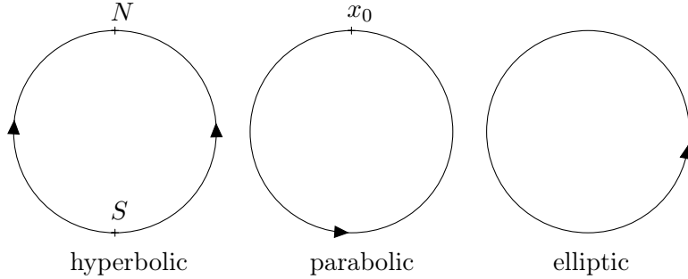
FIGURE 2.1. Dynamics of elements of \mathrm{PSL}(2, \mathbb{R})
