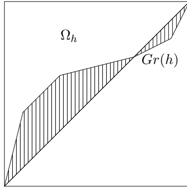
FIGURE 3.1. \Omega_h
