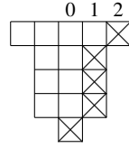
Fig. D.2 Decomposition into \mathfrak{sl}_2 -modules for (3, 1)
