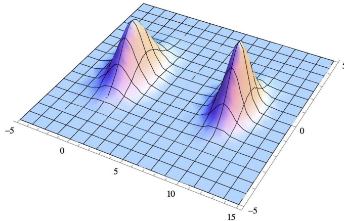
FIGURE 2. Aspect of the density of the trace \text{tr} U_n of a random unitary matrix, with U_n \sim \text{Haar} for the left peak, and U_n \sim \mu_{t < t_{\text{cut-off}}} for the right peak (using Mathematica ).
