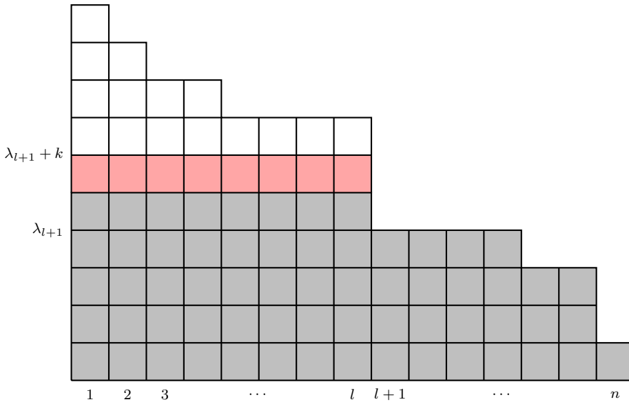
FIGURE 3. One makes the partitions grow layer by layer, starting from the bottom.
