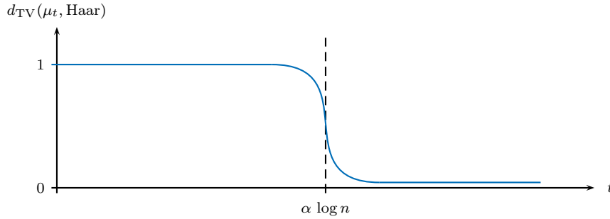
FIGURE 1. Aspect of the function t \mapsto d_{\text{TV}}(\mu_t, \text{Haar}) for the Brownian motion on a classical simple compact Lie group or on a classical simple compact symmetric space.
