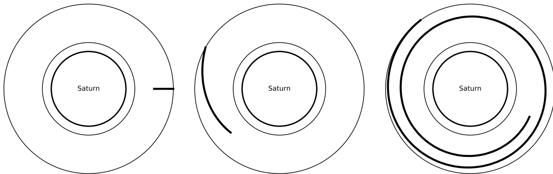
Figure 1: Equirepartition of a cloud of dust in Saturn's rings. On the left: the cloud (thick black line) at initial time. In the middle: the same cloud, after 6 hours. On the right: the same cloud, after 48 hours.
