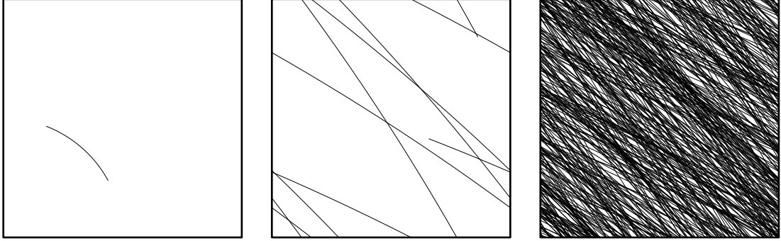
Figure 2: Propagation of a wavefront at unit speed in a unit square torus. The wave starts from the corner, and propagates at unit speed. On the left: the wavefront at time 0.5. In the middle: the wavefront at time 10. On the right: the wavefront at time 500.
